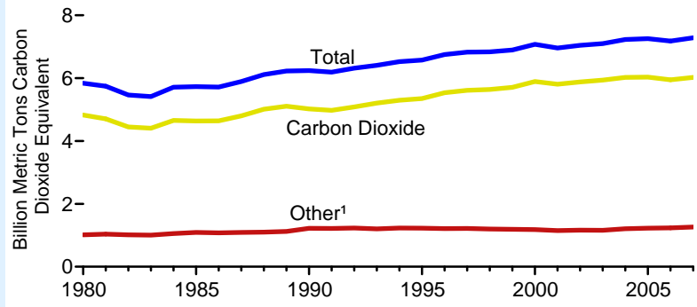
Figure 64. Greenhouse Gas Emissions, Based on Global Warming Potential
