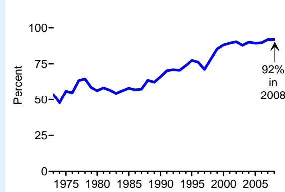
Figure 53. Nuclear Capacity Factor
